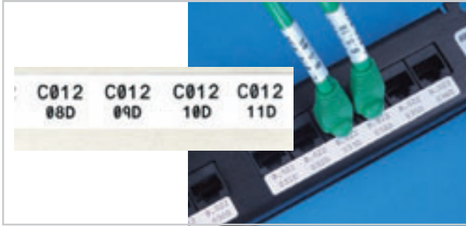
PATCH PANEL
